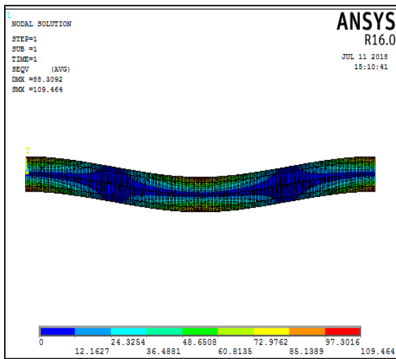
Fig 4: Bending Stress Results in Pipeline
